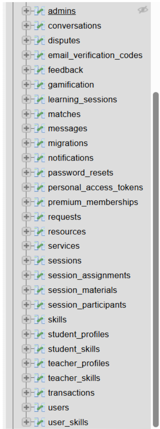
Figure 45: Database table
