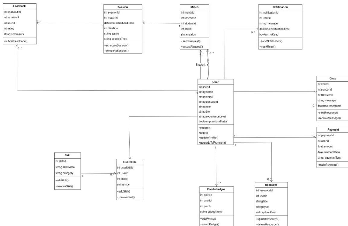
Figure 26: Class Diagram
