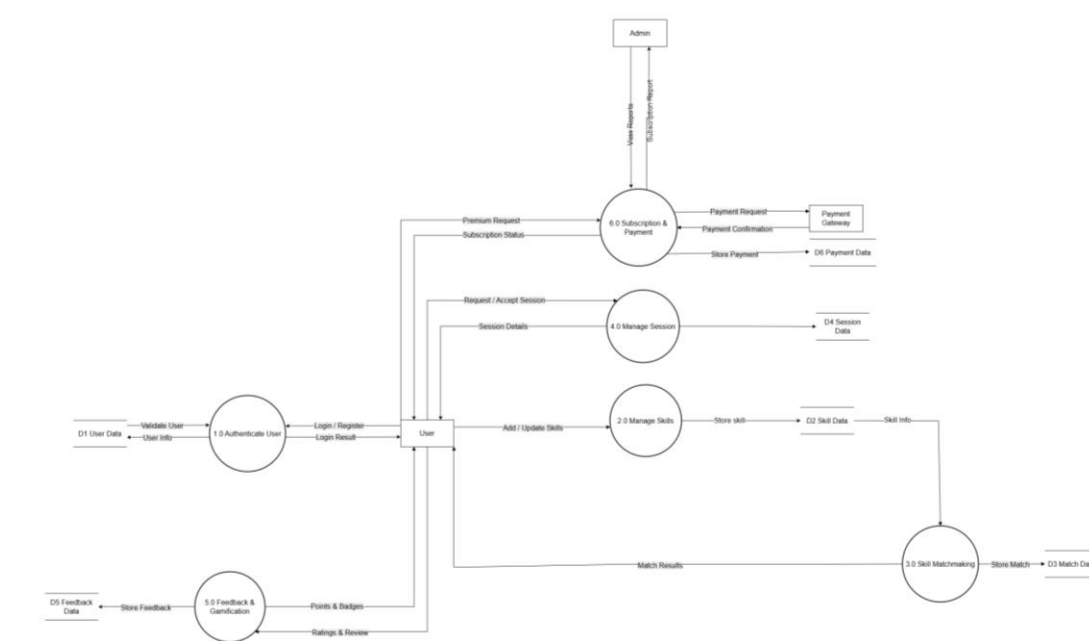
Figure 32: DFD1
