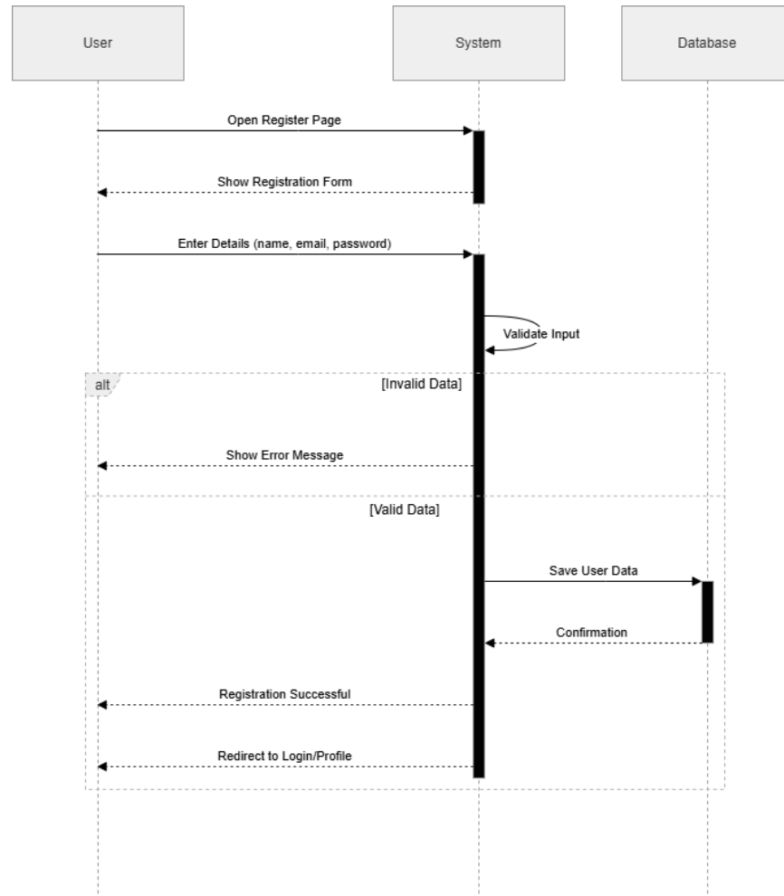
Figure 27: Sequences Diagram
